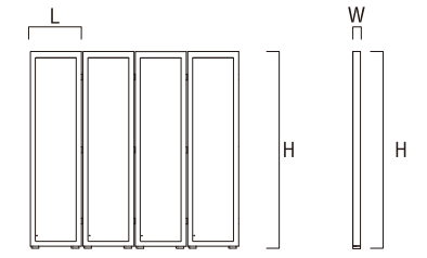
ITEM:Partition-3 CODE:O81003 SIZE:L600×W30×H2000mm*4
